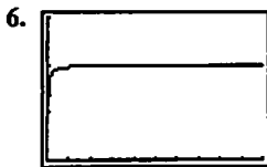
[0, 500] by [0, 3]
