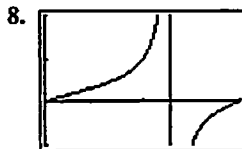
[0, \pi ] by [-1, 2]
