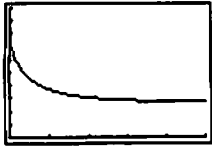
[0, 5] by [0, 10]
