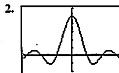
[-2, 2] by [-2, 6]
