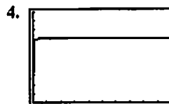
[0, 1000] by [0, 1]
