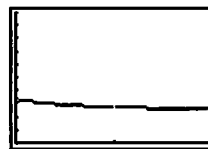
[0, 2] by [0, 1]
