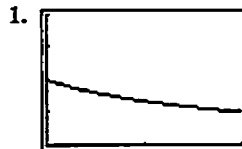
[0, 2] by [0, 1]
