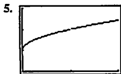
[0, 2] by [0, 3]
