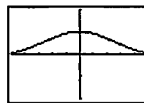
[-5, 5] by [-1, 1]
